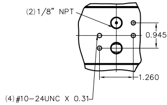
FS032 SIDE VIEW
