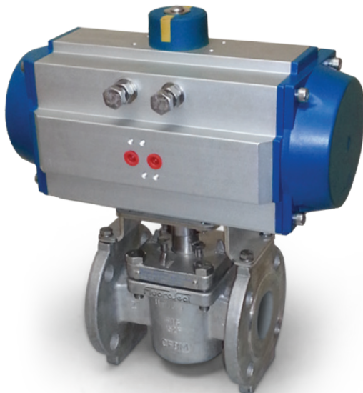
FluoroSeal FS095 Actuator mounted on a FluoroSeal Plug Valve
