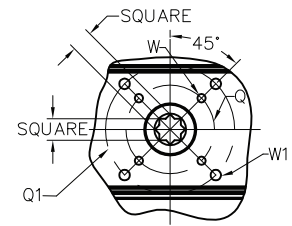
FS050-FS160 BOTTOM VIEW
