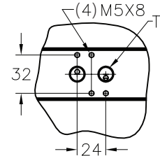
FM050-FM160 SIDE VIEW
