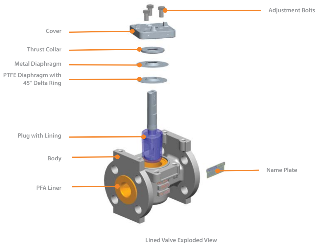
Lined Valve Exploded View
